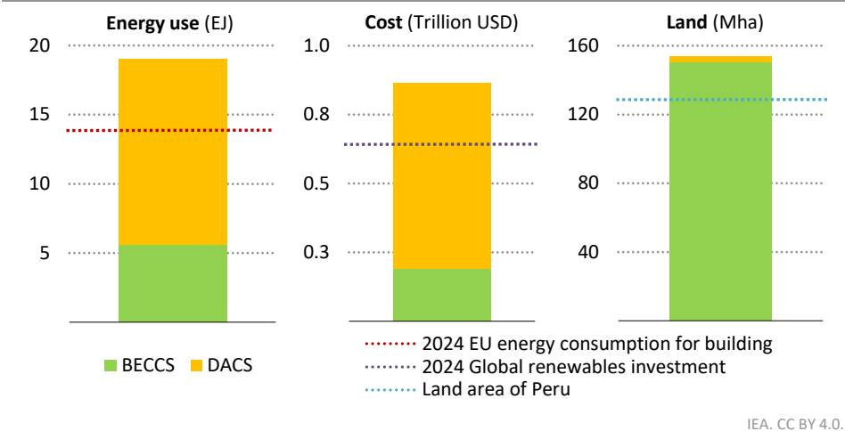
Figure 7.9 ▶ Global annual energy use, costs and land-use requirements for CO 2 removal technologies in the NZE Scenario, 2100
